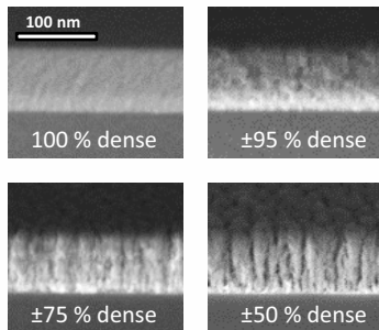
Full dense to textured porous thin films (Cross section SEM ZrO_2 )
